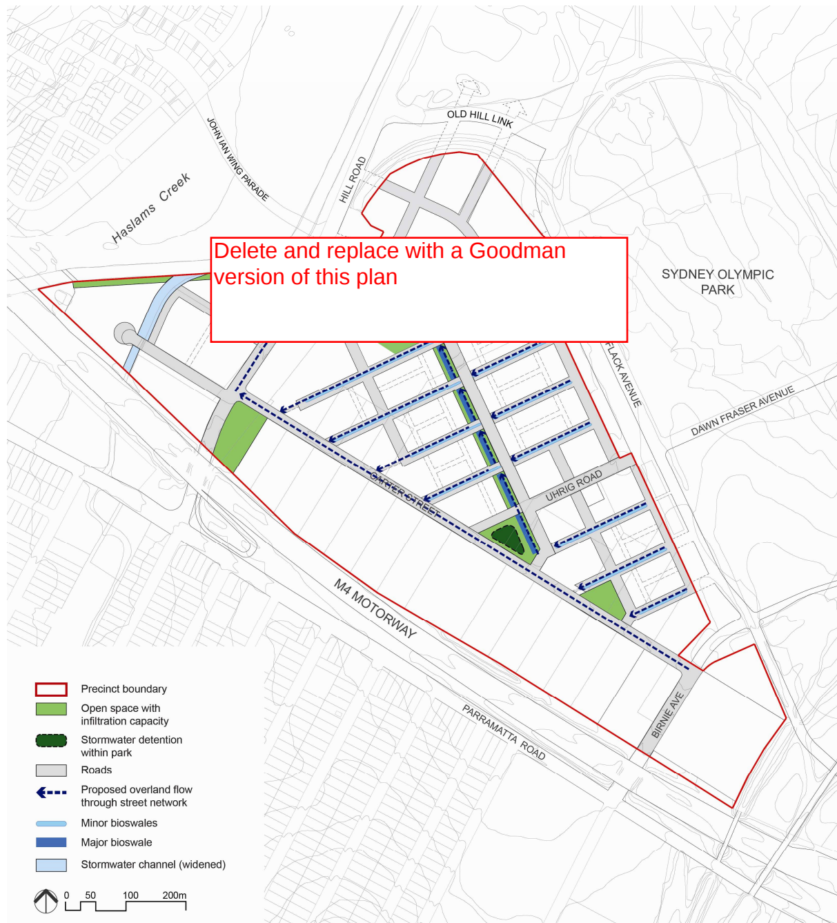
Figure 13 Indicative stormwater management
