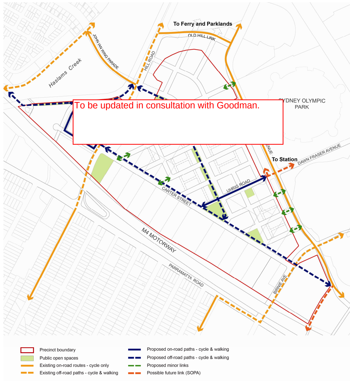
Figure 8 Pedestrian and cycle access
